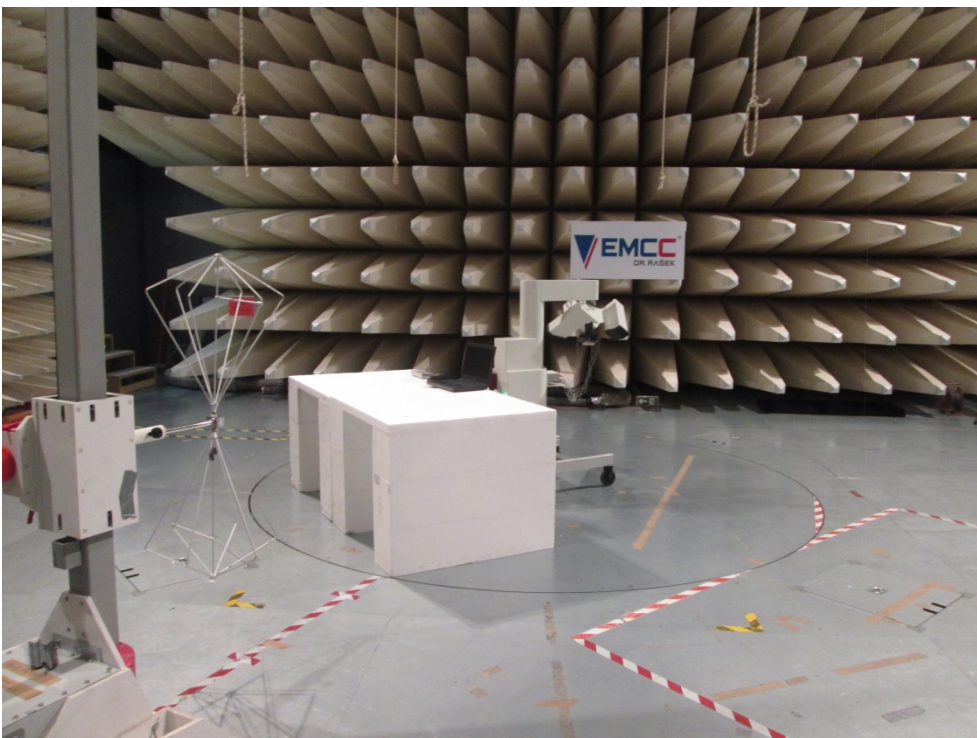
Photo A1-4: Radiated emissions measurement at 3 m distance, 30 MHz – 300 MHz
