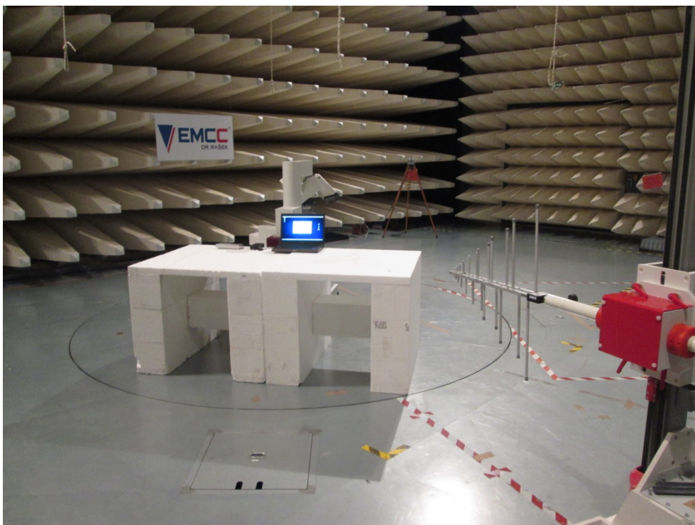
Photo A1-5: Radiated emissions measurement at 3 m distance, 300 MHz – 1000 MHz
