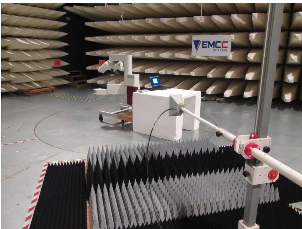
Photo A1-6: Radiated emissions measurement at 3 m distance, 1 GHz – 5 GHz
