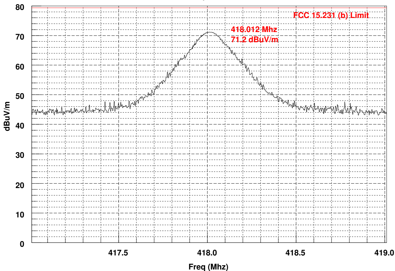
Waterleak X Systems, LLC Wireless Controller Model: 2AHFR-SRTS005 FCC 15.231 Amplitude Measurement
