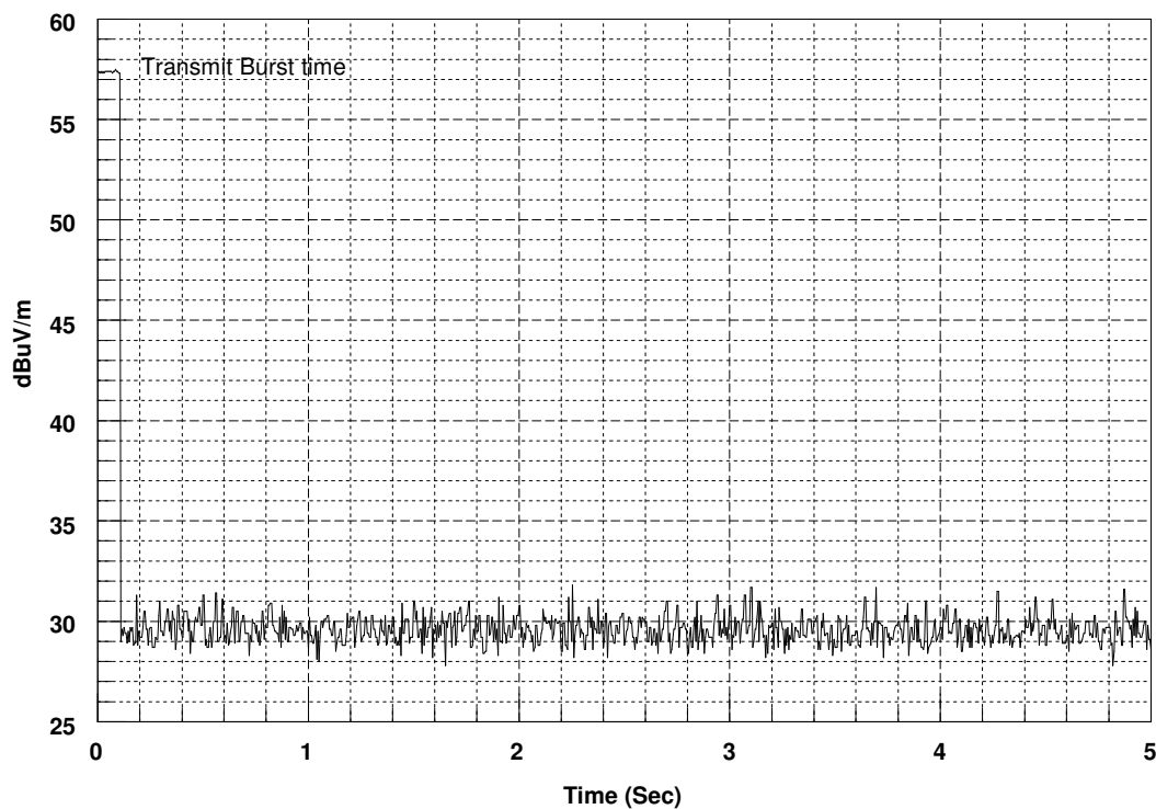
Waterleak X Systems, LLC Water Detection Unit Model: WDU003 Transmit Burst Time
