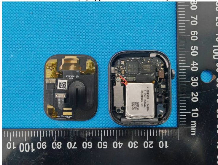
Model: GTX12(equipped with motor 1+Speaker 1)
