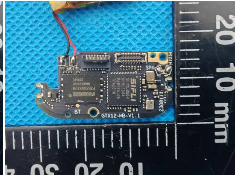
RF Chip
