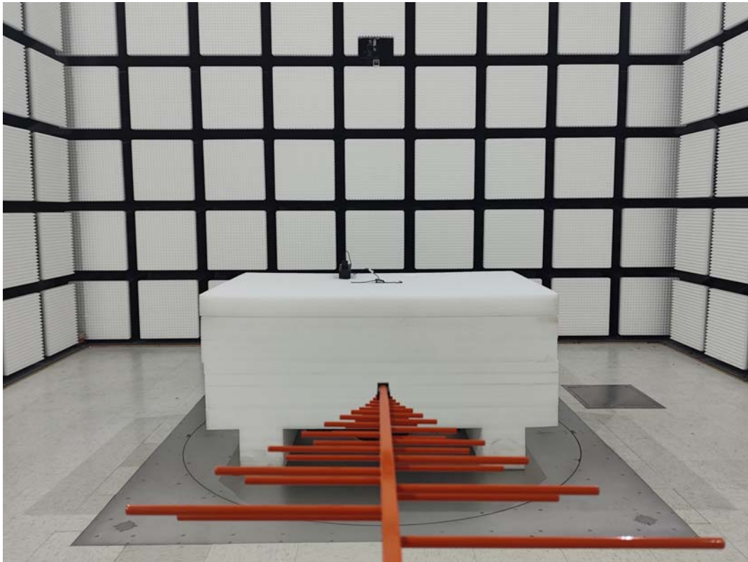
Radiated Emission Below 1GHz View Motor 2
