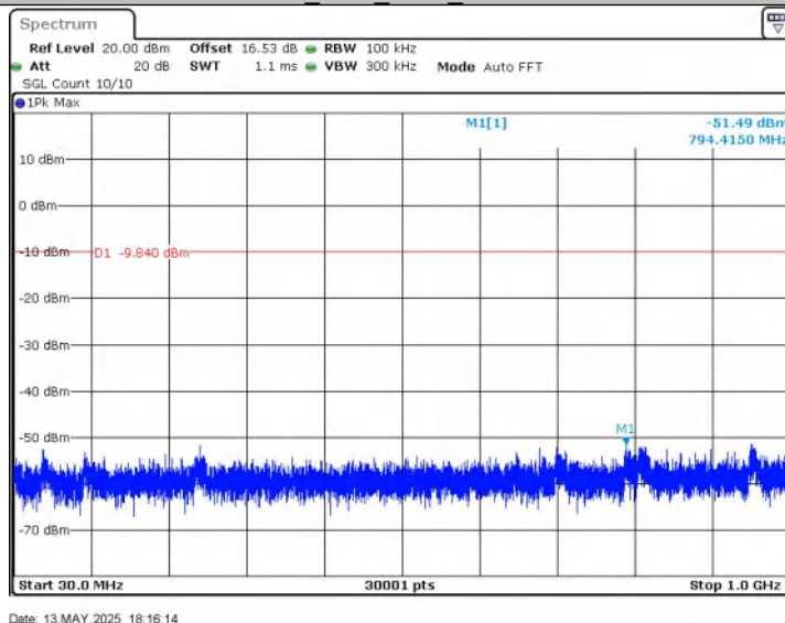
2DH5_Ant1_2480_30~1000
