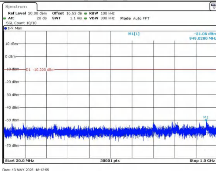
2DH5_Ant1_2441_30~1000
