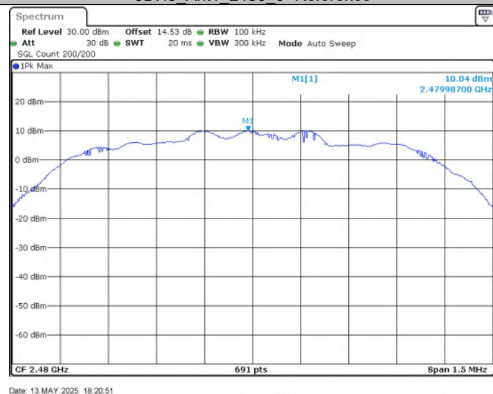
3DH5_Ant1_2480_0~Reference
