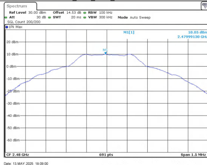
DH5_Ant1_2480_0~Reference
