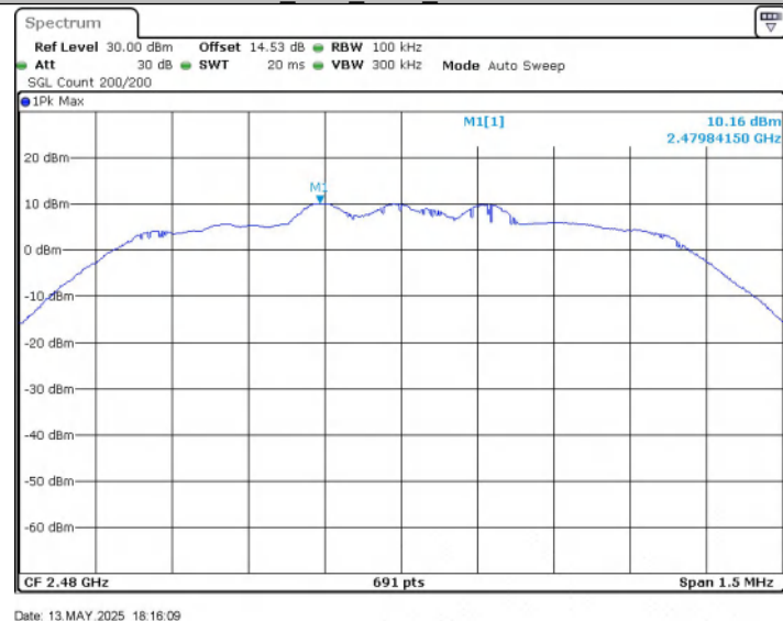
2DH5_Ant1_2480_0~Reference
