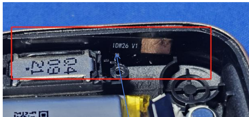
ANT Main control chip
