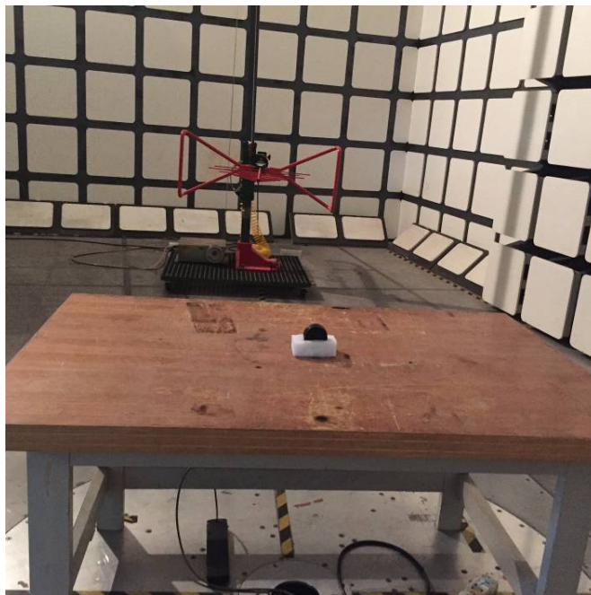
Radiated Emissions View (30 MHz~1 GHz)
