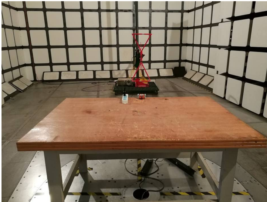
Radiated Emissions – Front View (Below 1 GHz) (Charging)
