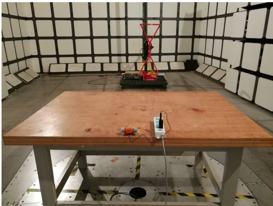
Radiated Emissions – Rear View (Below 1 GHz) (Charging)
