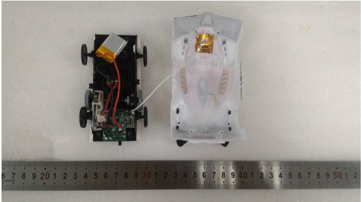
EUT – Cover off View
