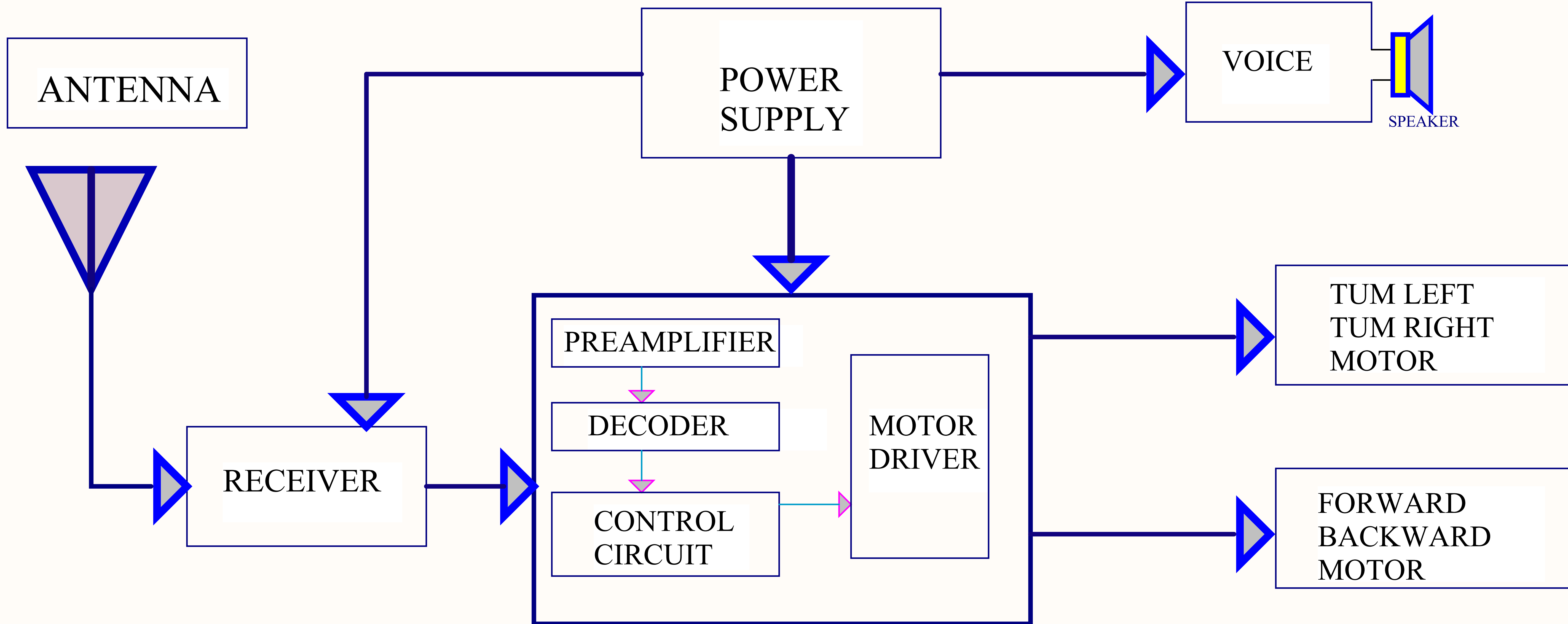
RX BLOCK DIAGRAM
