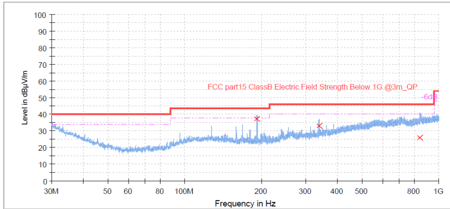
Figure 11: Spectral Diagrams, Radiated Emission, Mode A.3
