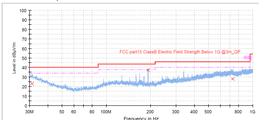
Figure 10: Spectral Diagrams, Radiated Emission, Mode A.2
