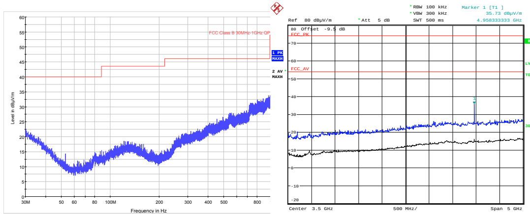
9 – Top Channel (30 MHz to 1 GHz).
