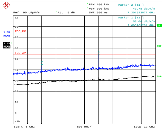
3 – Bottom Channel (6 GHz to 12 GHz).
