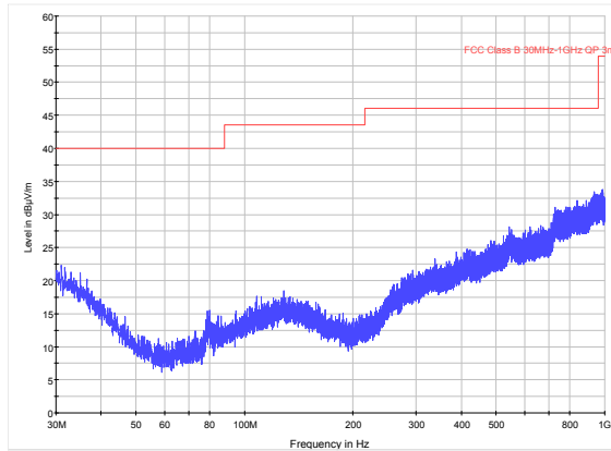
1 – Bottom Channel (30 MHz to 1 GHz).
