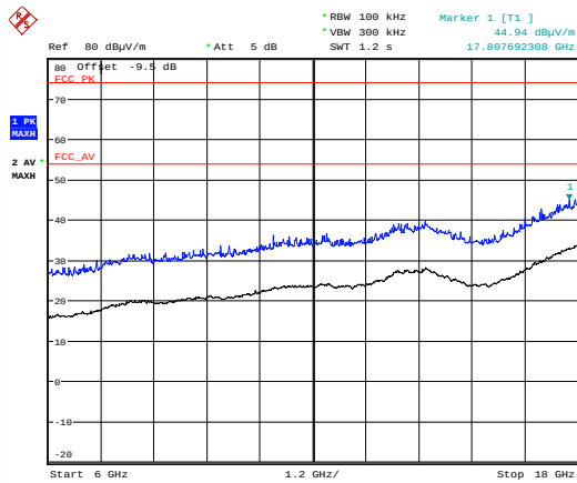
11 – Top Channel (6 GHz to 18 GHz).
