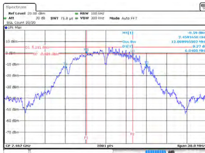
Minimum Emission Bandwidth Plots (6dB)
