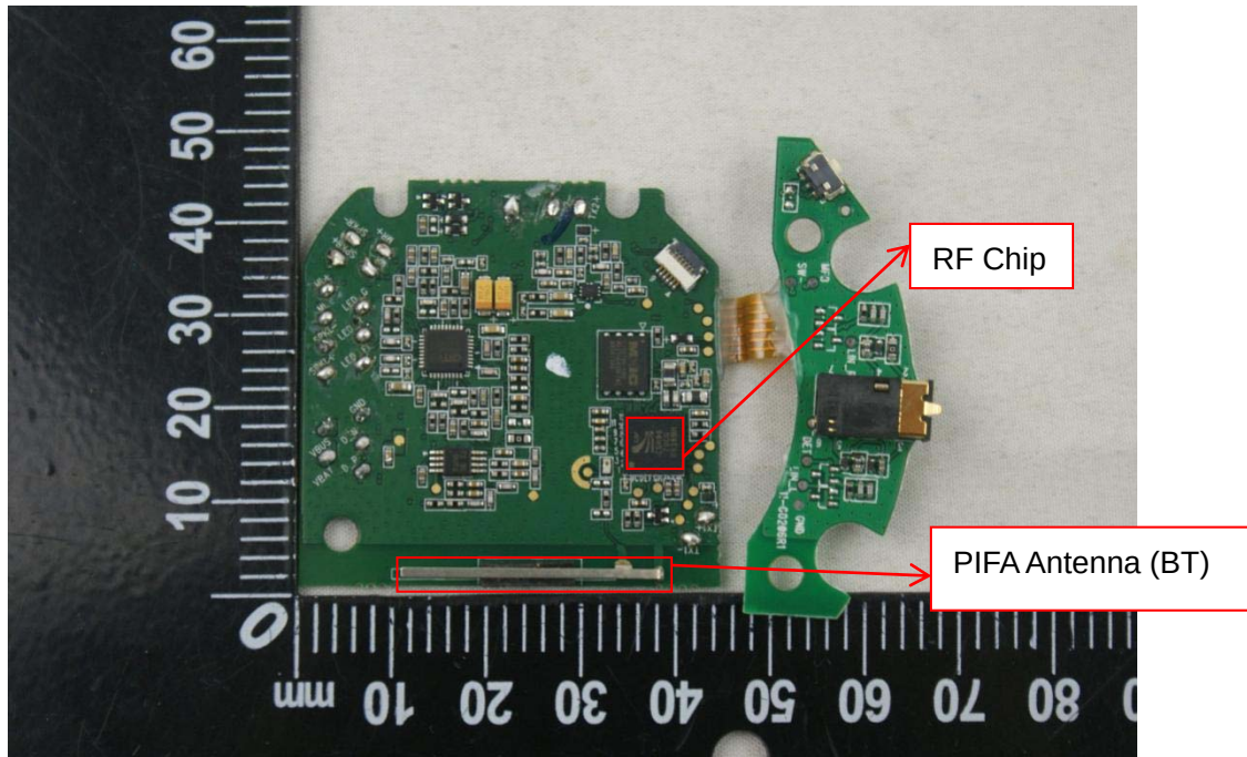
Mainboard front view 1
