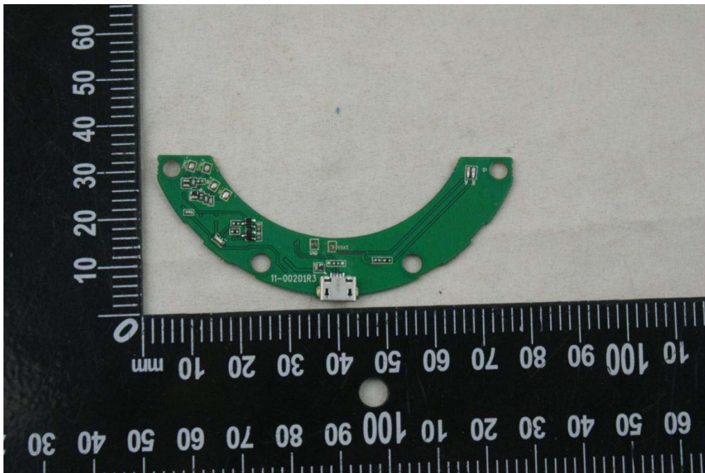
Mainboard rear view 2
