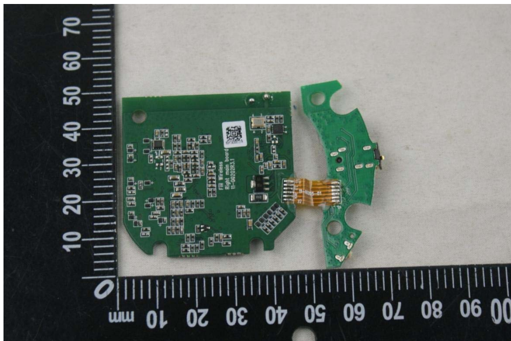
Mainboard rear view 1
