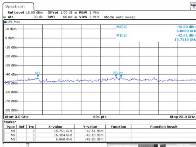
Middle CHANNEL, SPURIOUS 3 GHz ~ 25 GHz
