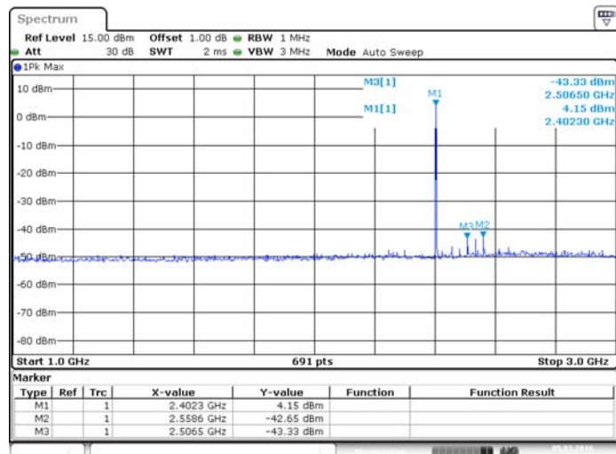
LOW CHANNEL, SPURIOUS 1 GHz ~ 3 GHz
