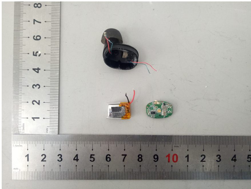
EUT – Right Earphone Battery View
