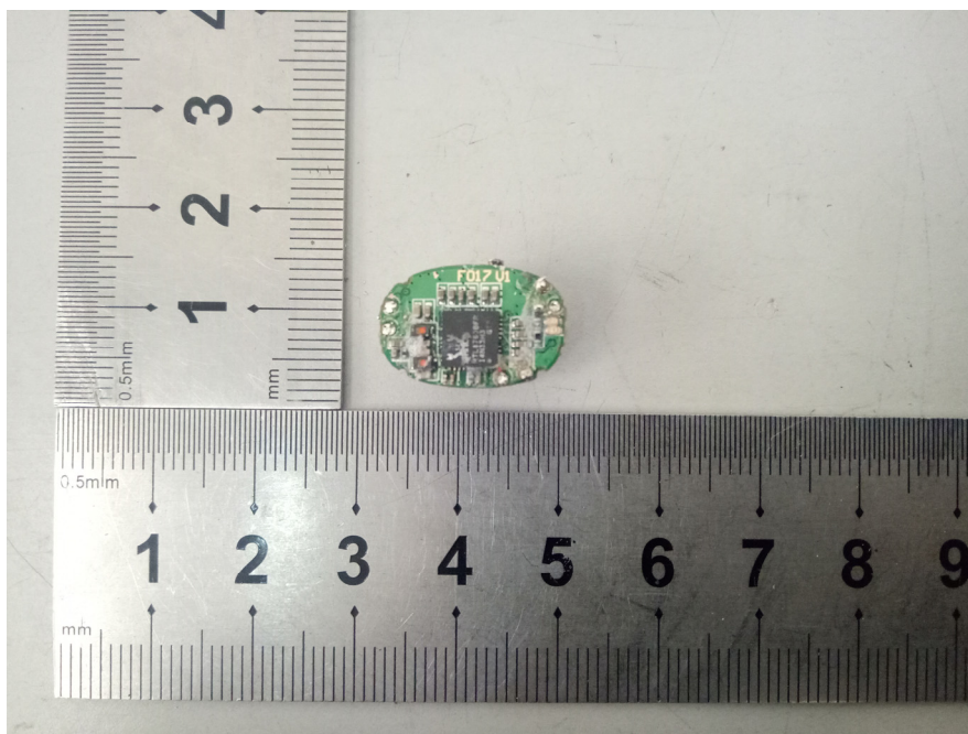
EUT – Right Earphone PCB Bottom View
