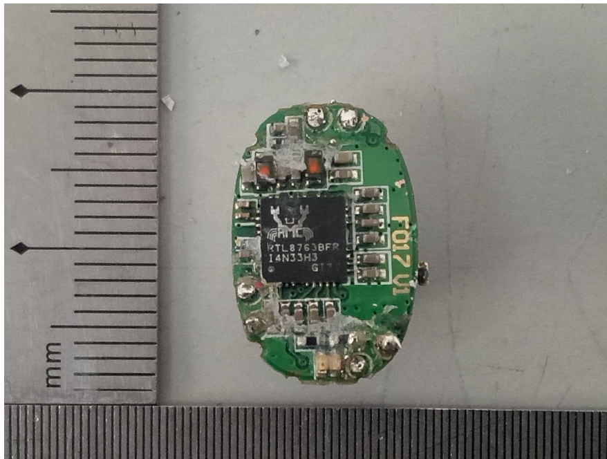
EUT – Right Earphone PCB IC Chip View
