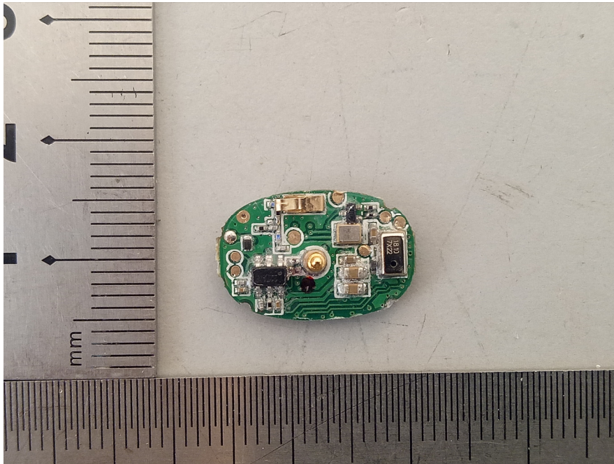
EUT – Left Earphone PCB Bottom View
