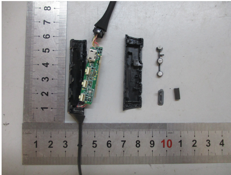
EUT – Left Earphone PCB Top View
