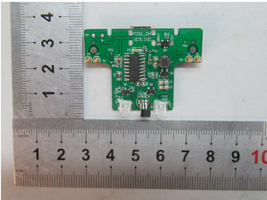
Charging Case – PCB Top View
