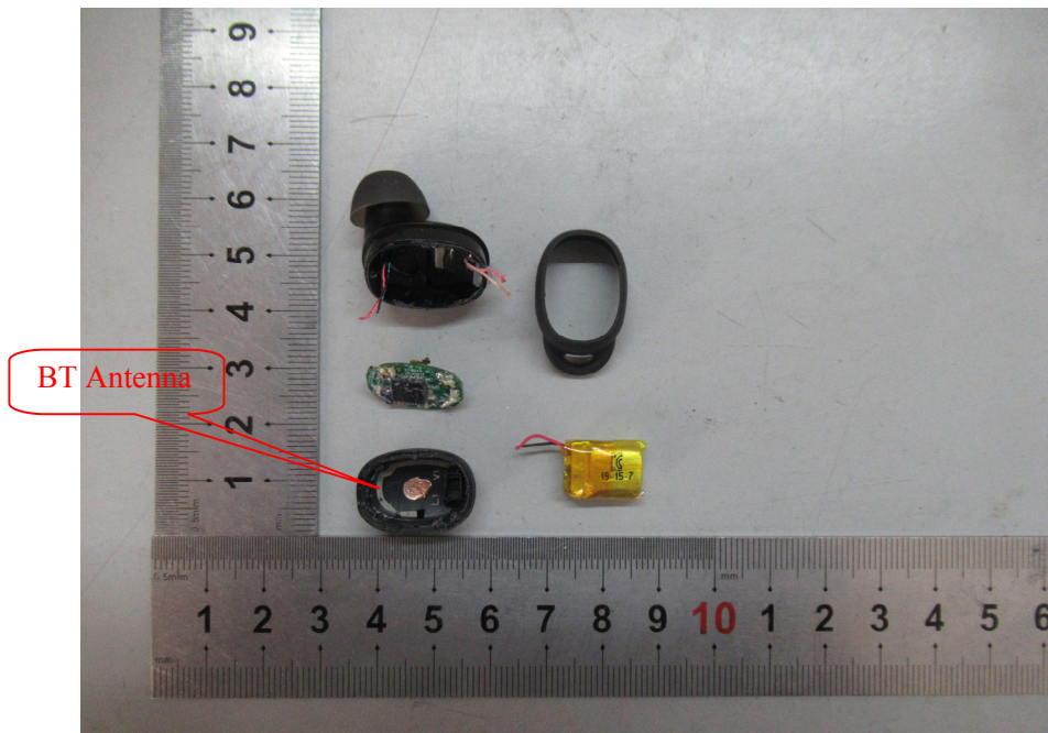
Earbuds(L) – Battery View
