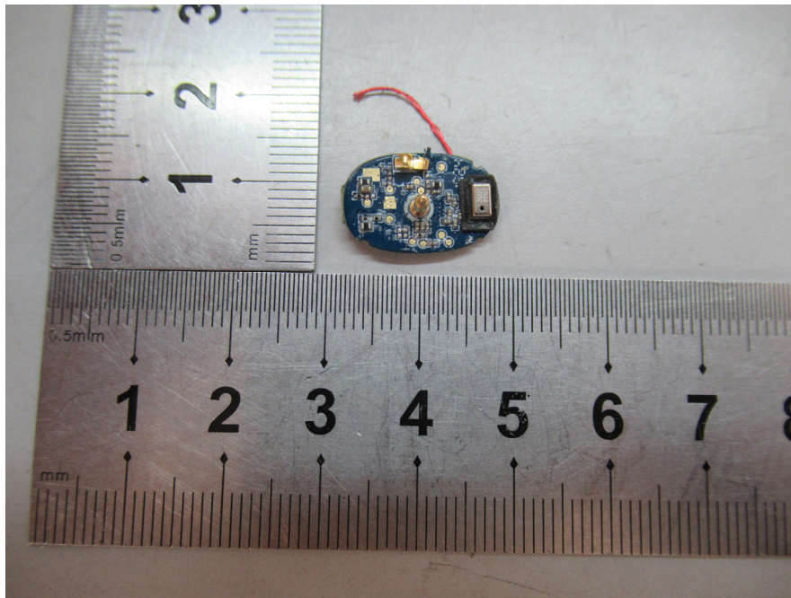
Earbuds(R) – PCB Bottom View
