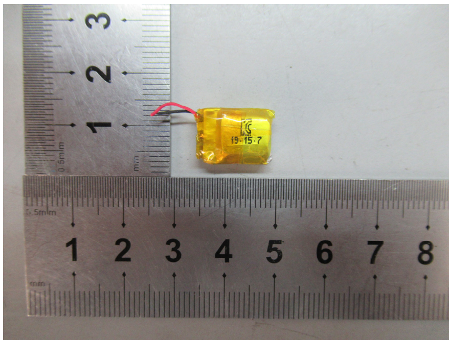
Earbuds(L) – Battery View
