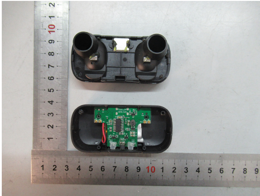
Charging Case – Cover off View-2
