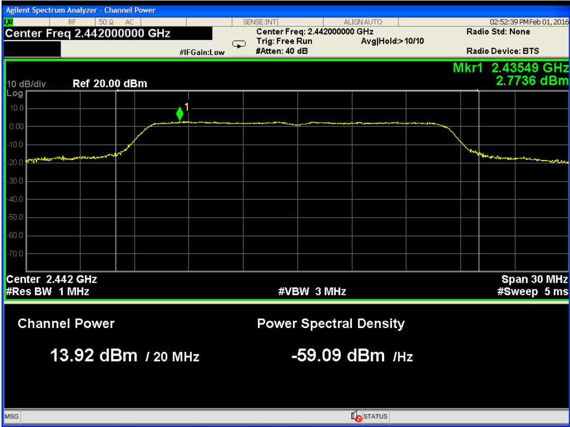
Channel 7: 2.442GHz:
