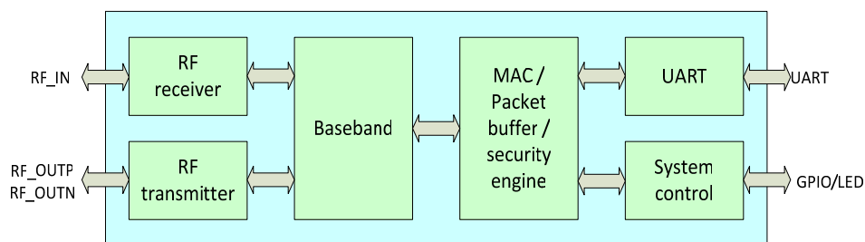
5005-HBS block diagram
