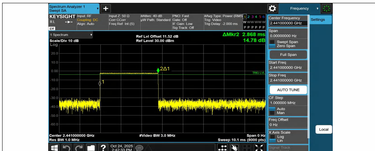
DH5-Ant1-Hop-PASS
