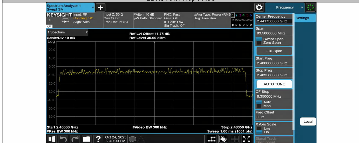
3DH5-Ant1-Hop-PASS
