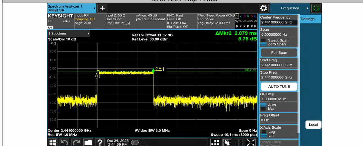
2DH5-Ant1-Hop-PASS
