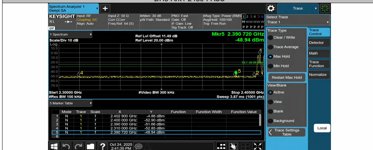
DH5-Ant1-Hop_2402-PASS
