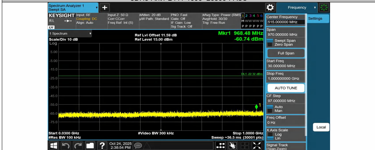
3DH5-Ant1-2480-30~1000-PASS
