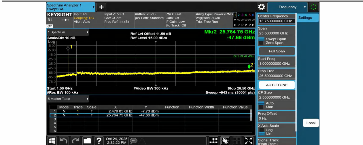
2DH5-Ant1-2480-1000~26500-PASS
