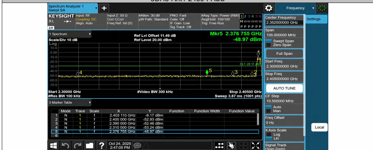
3DH5-Ant1-Hop 2402-PASS
