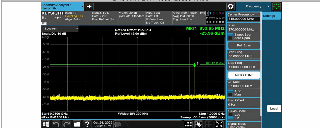
DH5-Ant1-2480-30~1000-PASS
