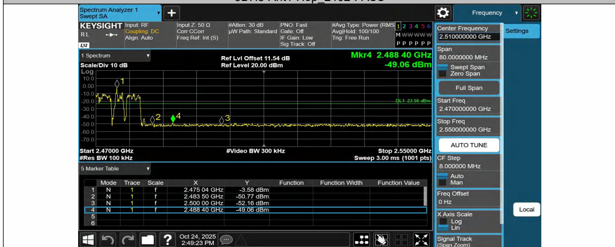
3DH5-Ant1-Hop 2480-PASS
