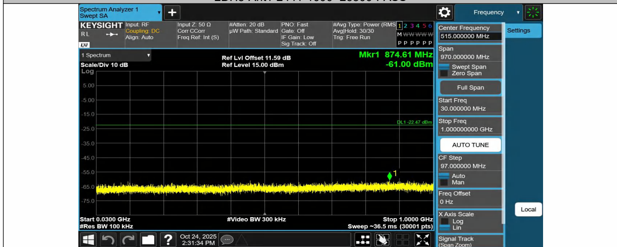
2DH5-Ant1-2480-30~1000-PASS
