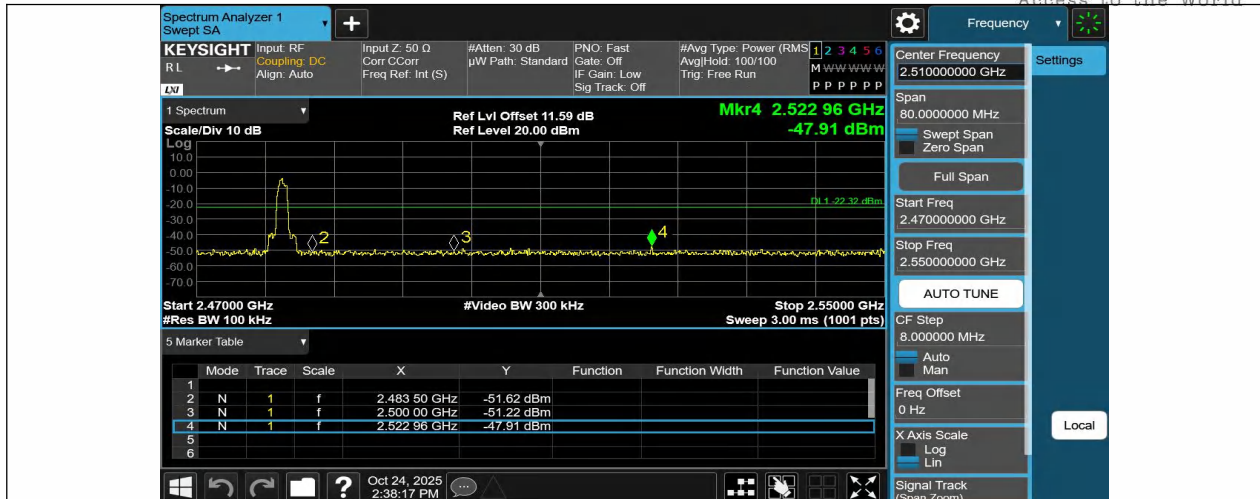
3DH5-Ant1-2480-PASS
