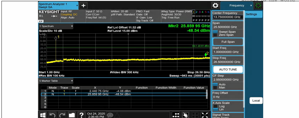
3DH5-Ant1-2441-1000~26500-PASS
