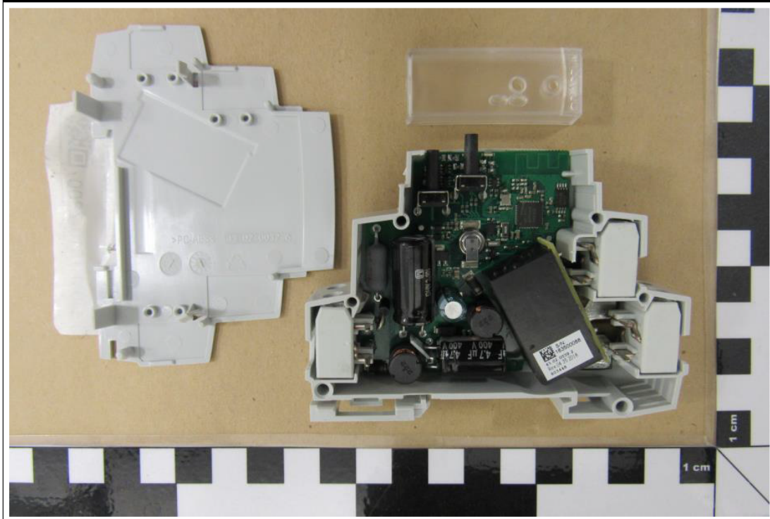
EUT INTERNAL VIEW (A)
