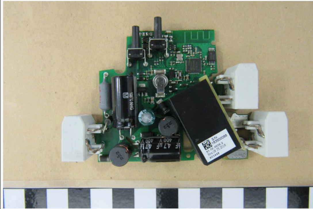
EUT INTERNAL VIEW (C)
