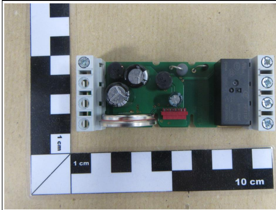
EUT C15 PCB II FRONT
