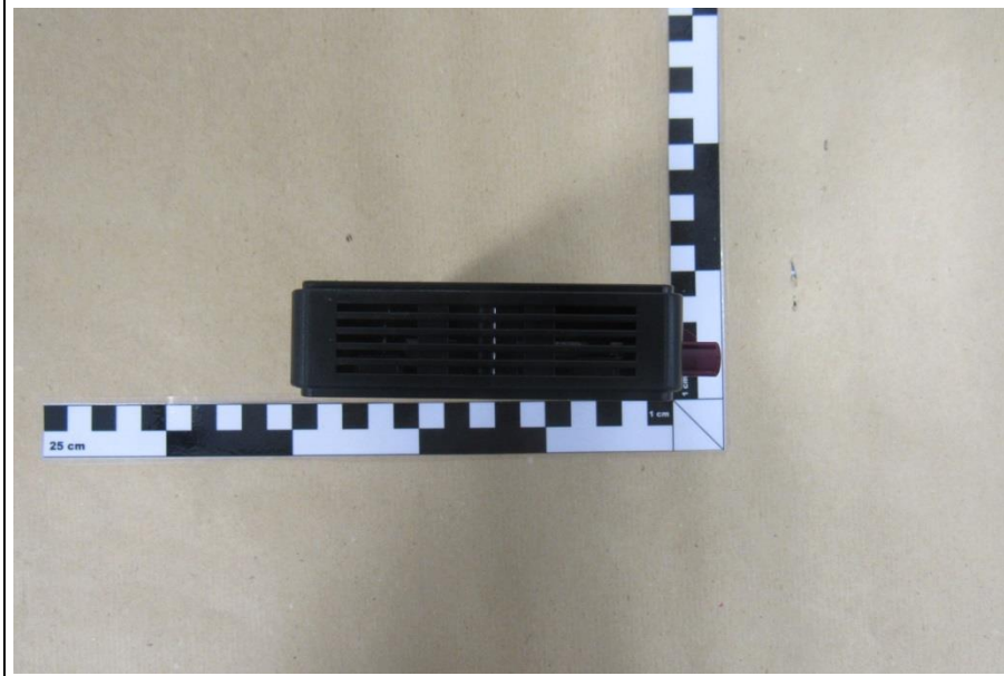
EUT-right side
