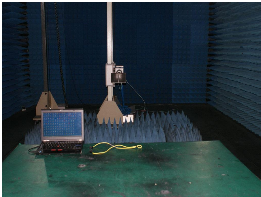
Photograph 6: Set-up for Radiated Emission (1GHz ~ 6GHz)
