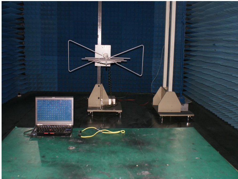
Photograph 5: Set-up for Radiated Emission (30MHz ~ 1GHz)
