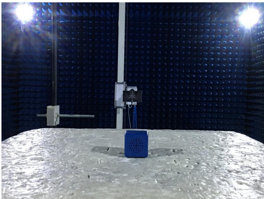
Set -up for Radiated Spurious Emission, 1GHz - 18GHz
