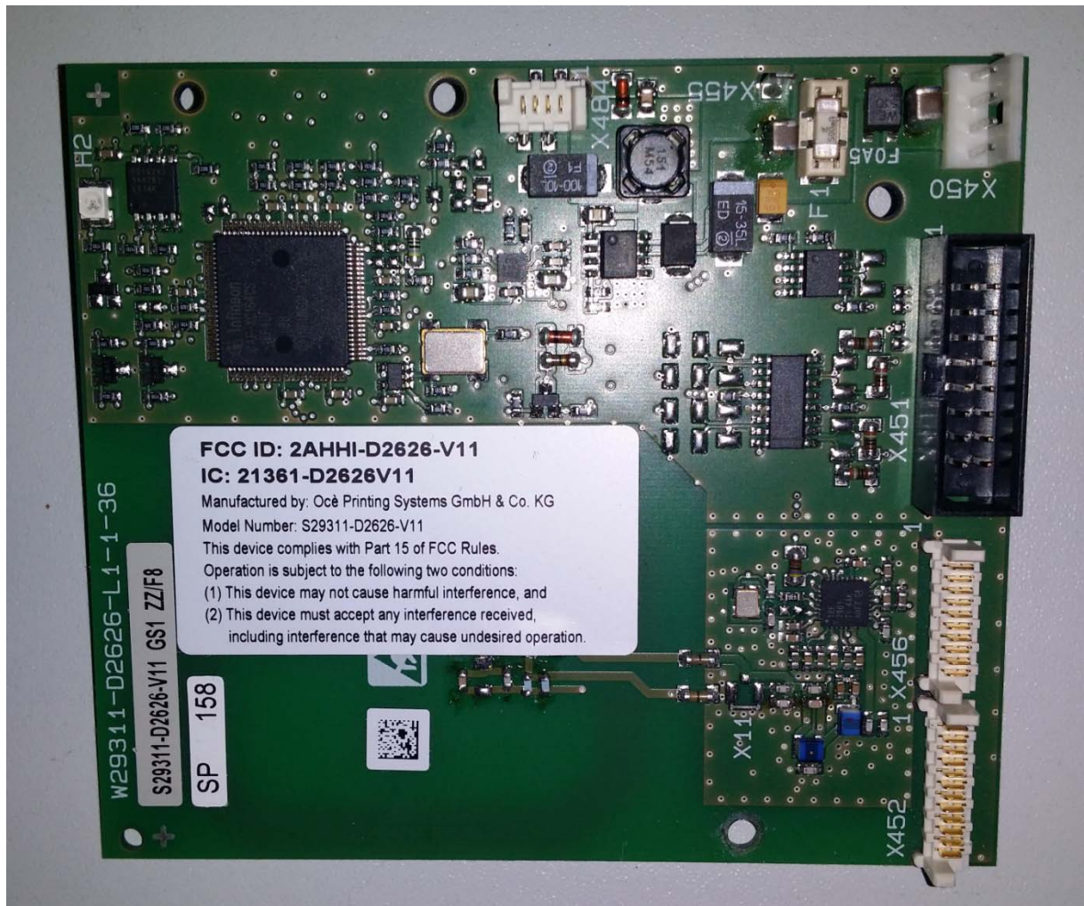
Figure 1: front side of S29311-D2626-V11
