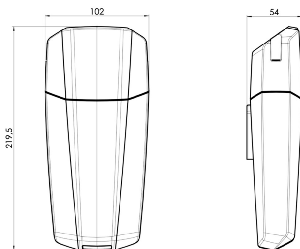
Figure 12 - Dimension of the CorivaSat (IP67 Version)
