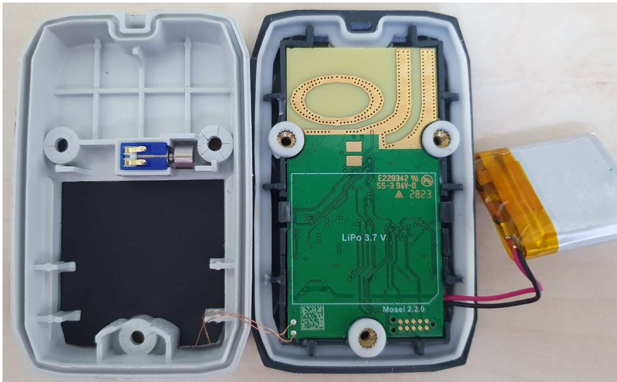
inside back view with LiPo off
