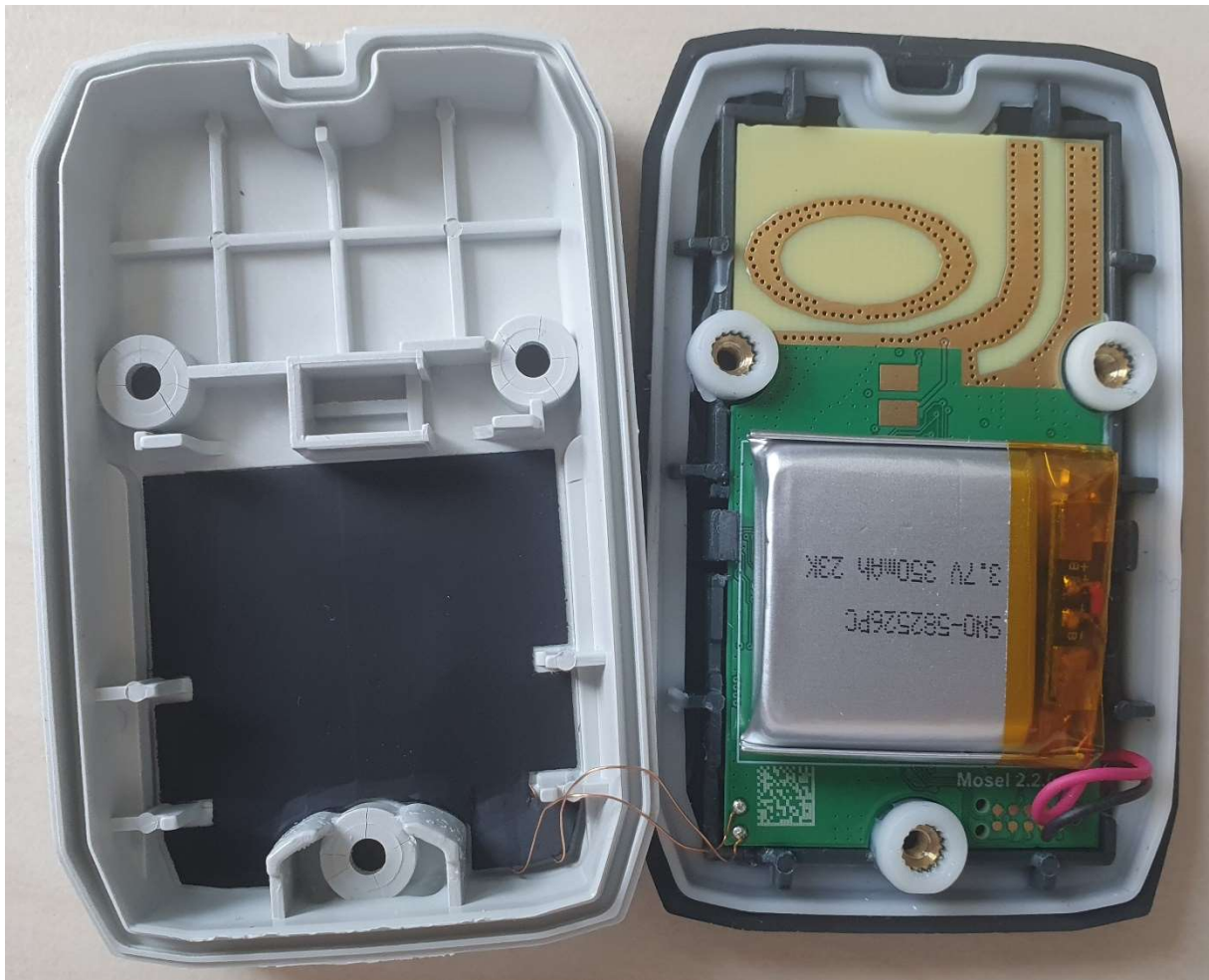
inside back view without vibration motor
