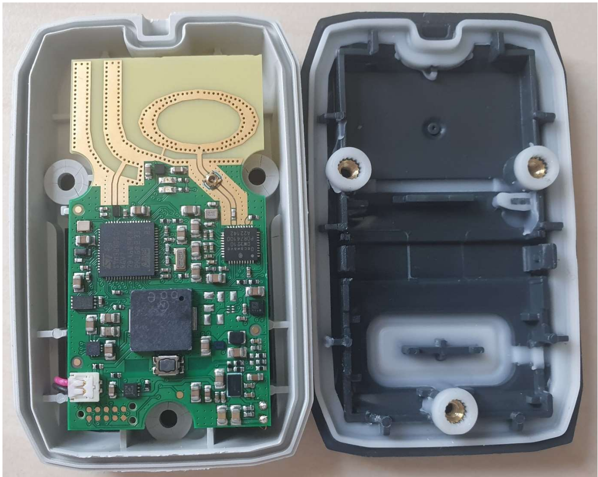
inside front view
