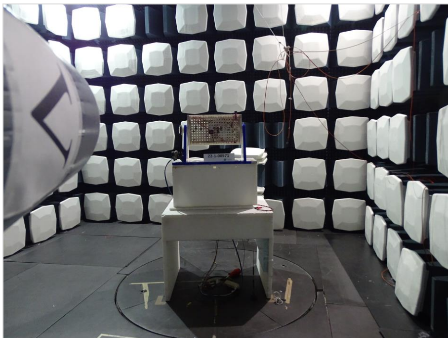
Photograph 8: EUT test setup in the fully anechoic chamber, overview_EUT elevation 0°
