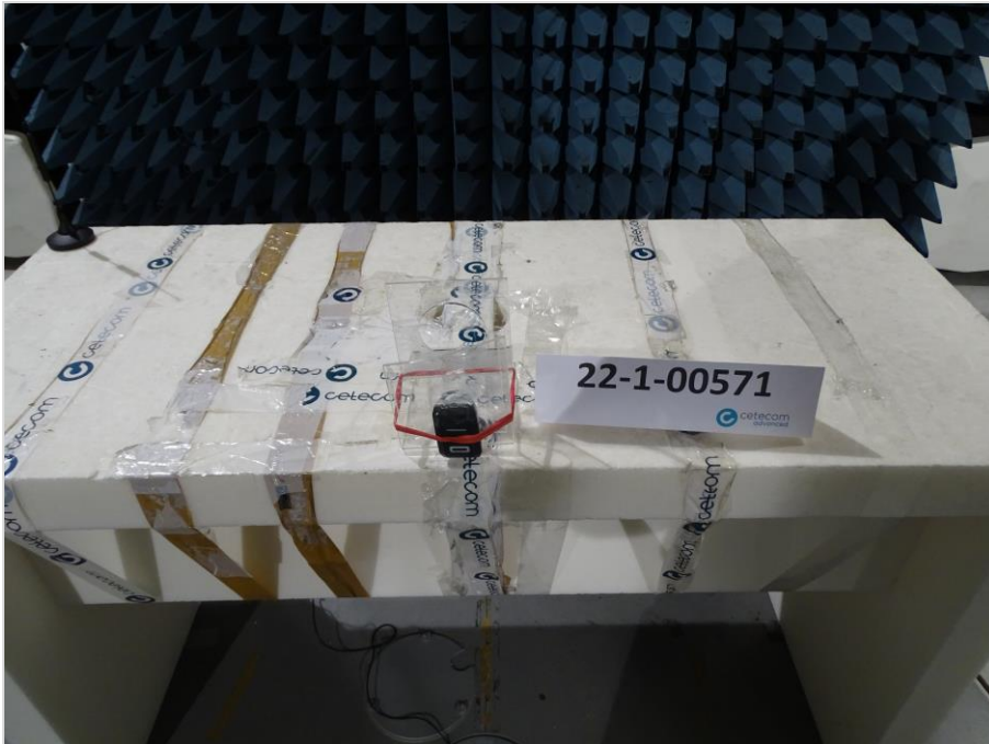
Photograph 3: EUT test setup in the semi anechoic chamber, close up view_EUT elevation 0°
