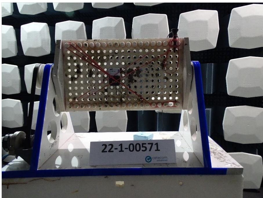
Photograph 7: EUT test setup in the fully anechoic chamber, close up view_EUT elevation 0°
