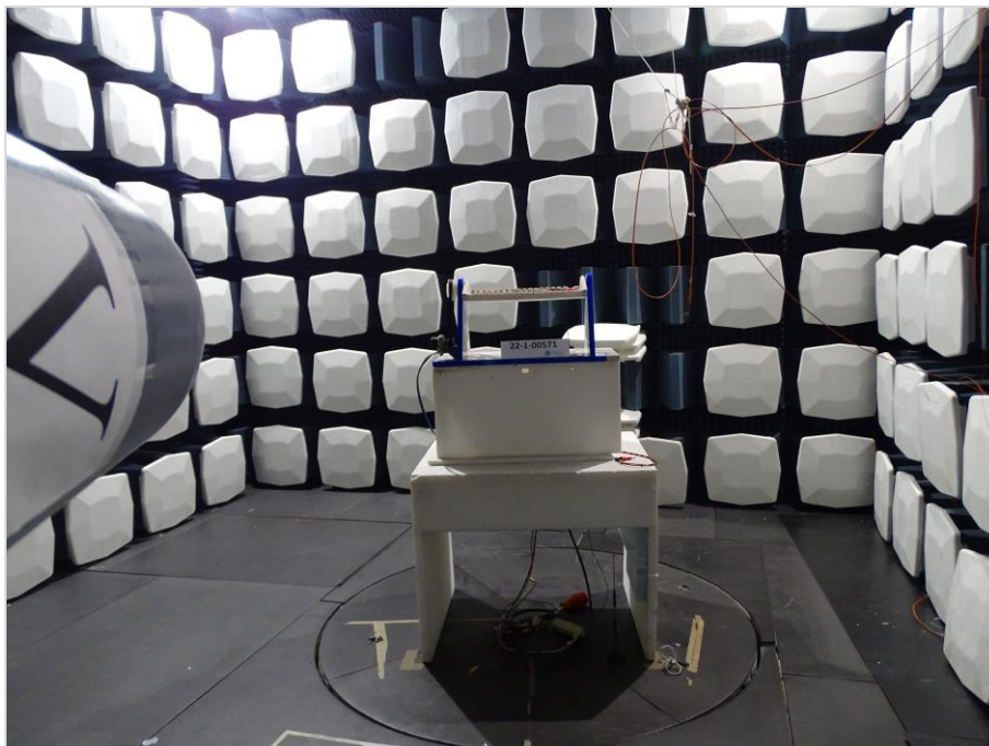
Photograph 10: EUT test setup in the fully anechoic chamber, overview_EUT elevation 90°
