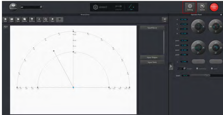
Figure 5.49 Click Setting
