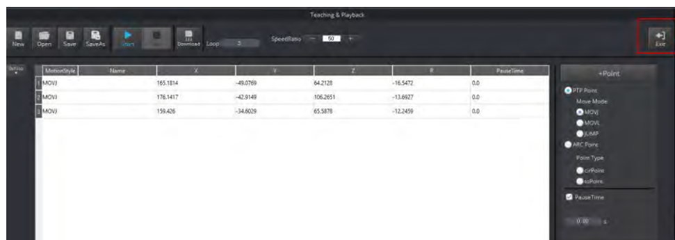
Figure 2.24 Click Exit
