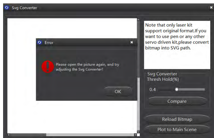
Figure 5.48 Error tip
