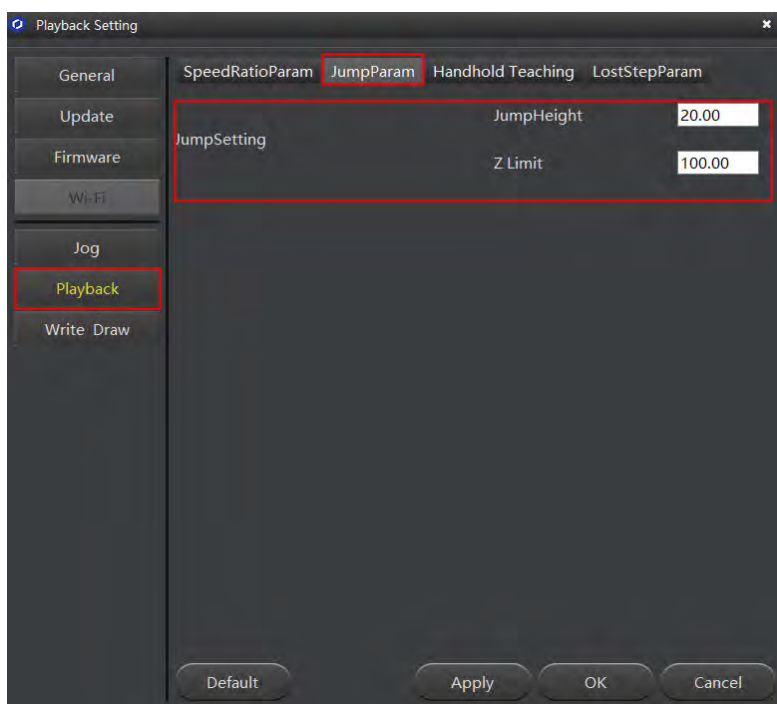
Figure 5.27 Jump parameters
