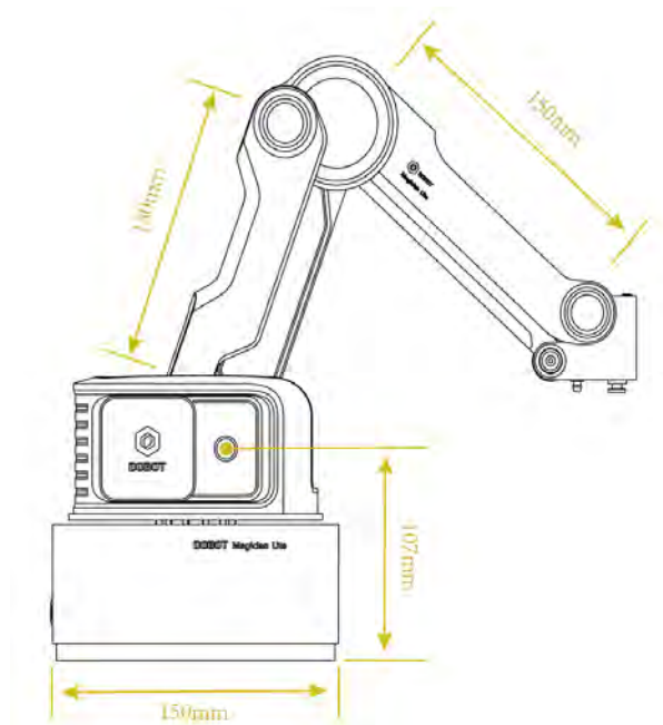
Figure 3.10 Size of Magician Lite
