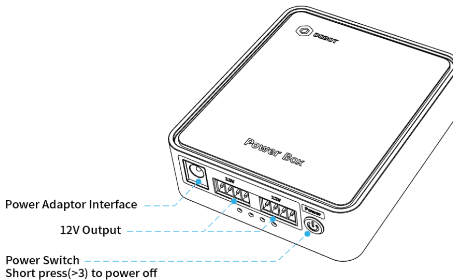
Figure 4.2 Power Box interface description
