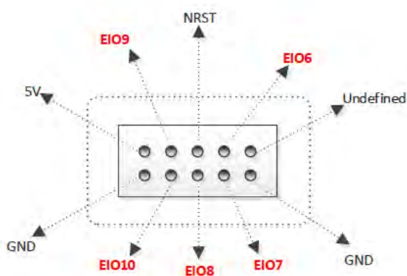
Figure 4.5 Communication Interface 2
