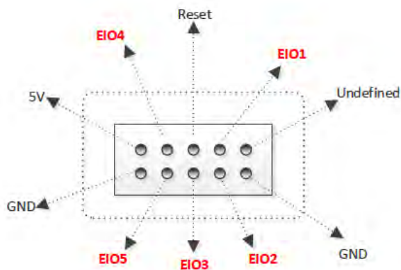
Figure 4.3 Communication interface
