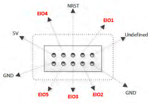
Figure 4.4 Communication Interface 1
