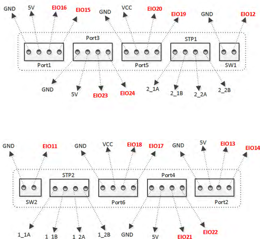
Figure 4.6 Peripheral interface
