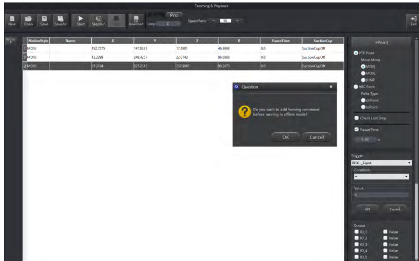
Figure 5.31 Click Download
