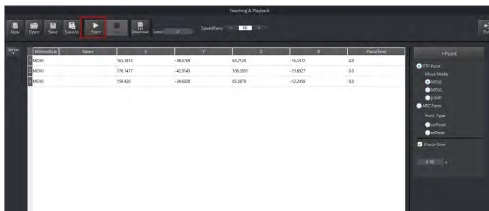
Figure 2.23 Click Start
