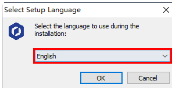
Figure 2.8 Select English
