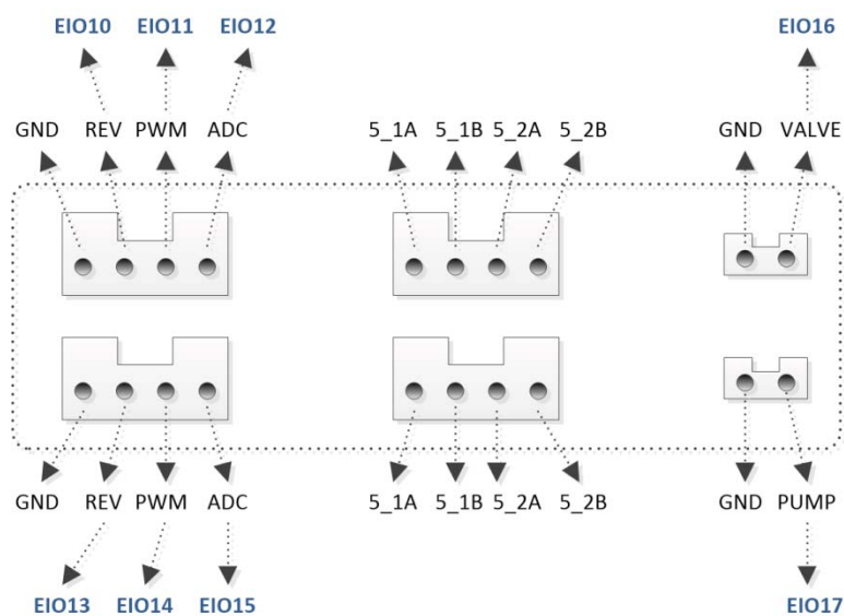
Figure 4.4 Peripheral Interface
