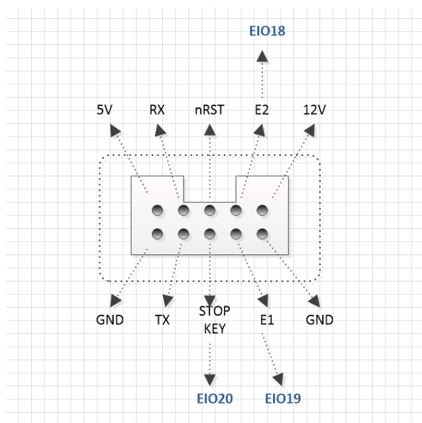
Figure 4.3 UART interface
