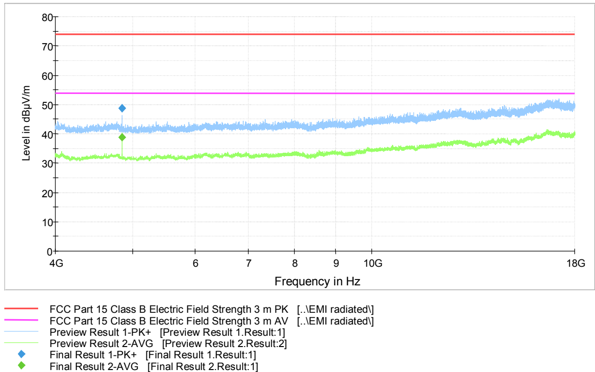
Figure 11. Measured curve with peak and average detectors (Mid channel).
