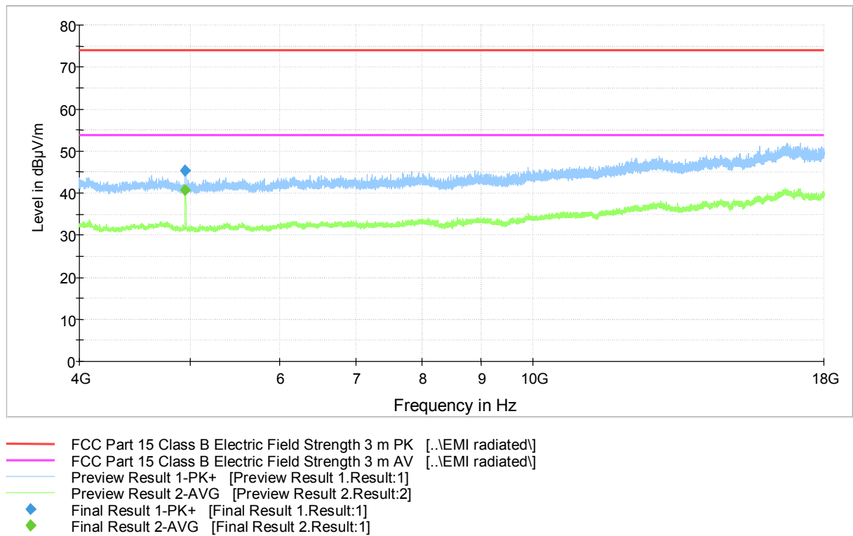
Figure 12. Measured curve with peak and average detectors (High channel).
