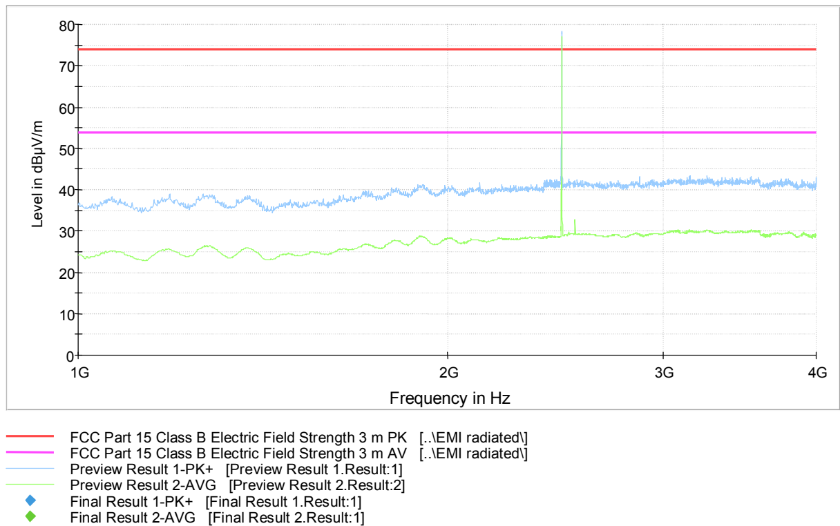
Figure 9. Measured curve with peak and average detectors (High channel).
