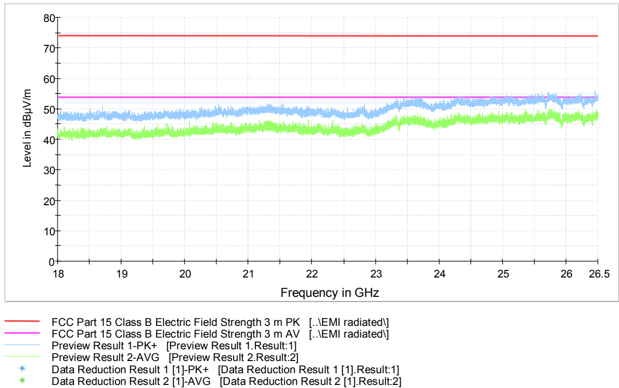
Figure 15. Measured curve with peak and average detectors (High channel).
