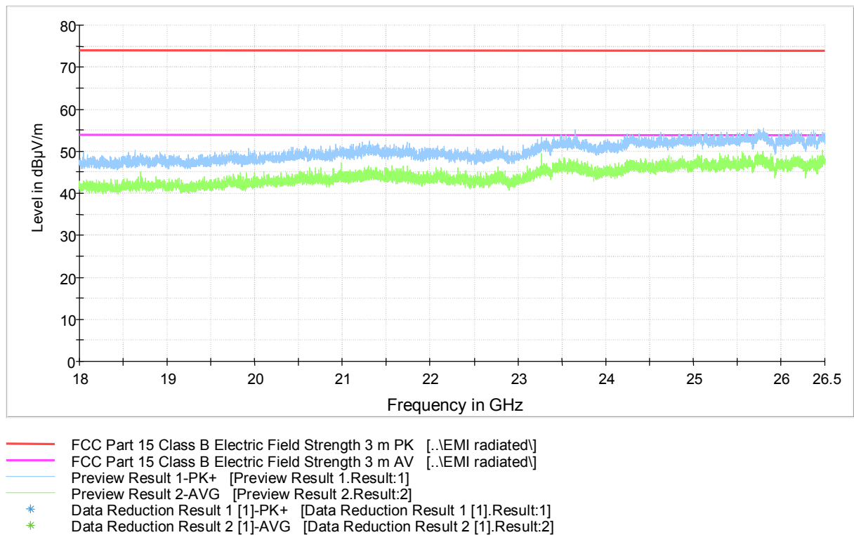
Figure 14. Measured curve with peak and average detectors (Mid channel).
