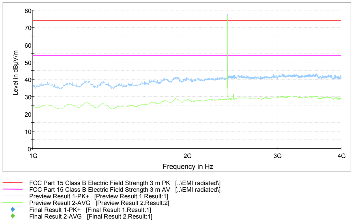
Figure 7. Measured curve with peak and average detectors (Low channel).
