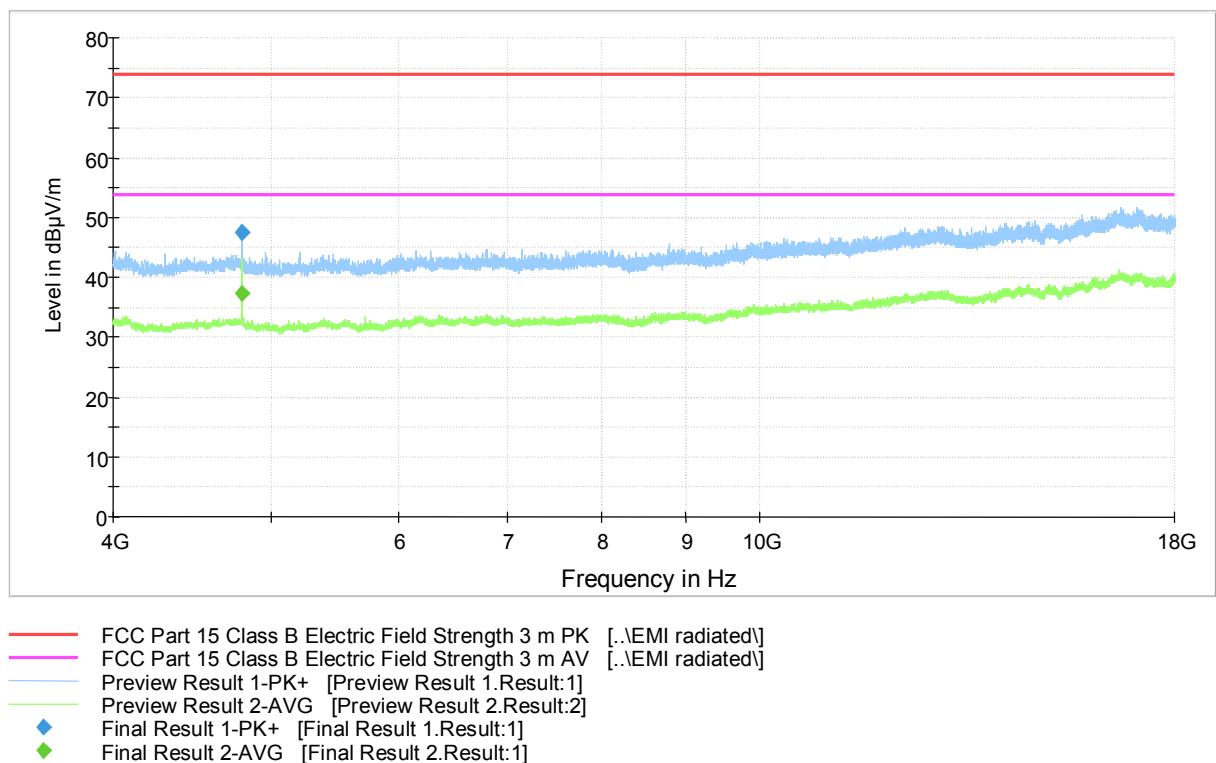
Figure 10. Measured curve with peak and average detectors (Low channel).
