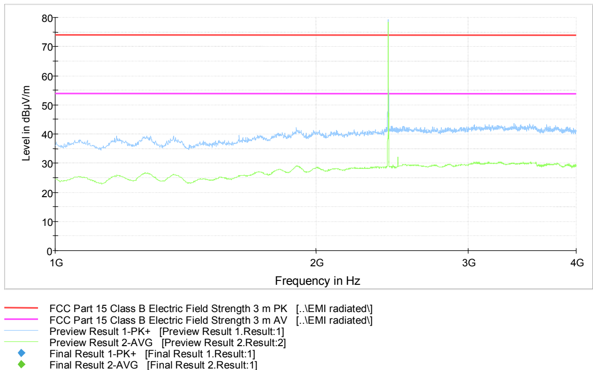
Figure 8. Measured curve with peak and average detectors (Mid channel).
