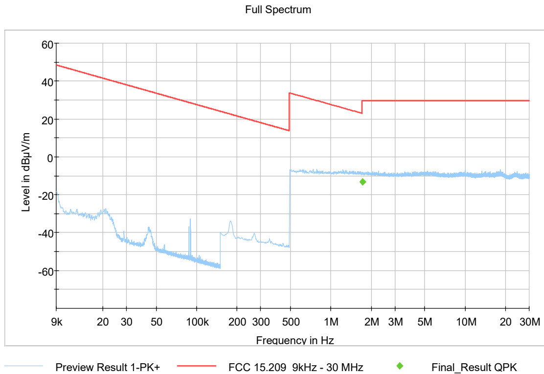
Figure 2. Measured curve with peak detector (Low channel).
