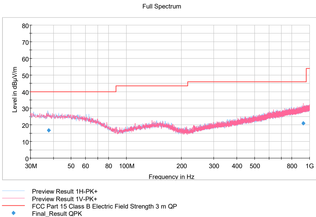
Figure 3. Measured curve with peak detector (High channel).
