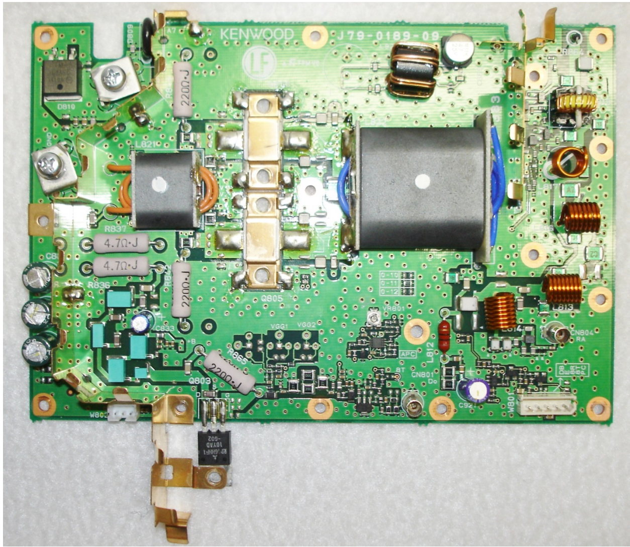
RF PA BOARD
