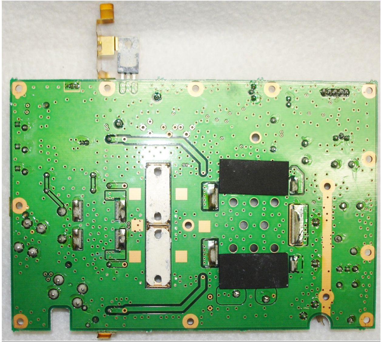
RF PA BOARD
