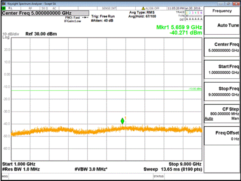
(Channel 128: 824.20MHz @ Traffic @ GSM850)
