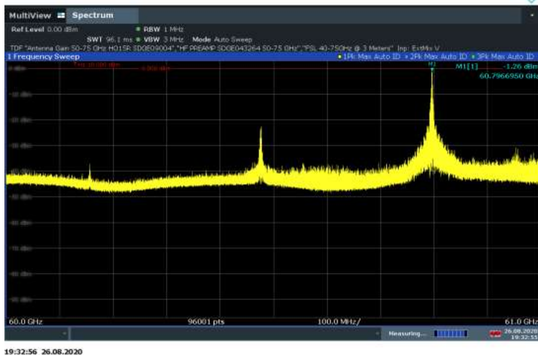
60GHz to 61GHz Plot (12 Transmitters)
