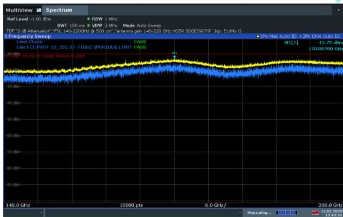
140GHz to 200GHz Plot (24 Transmitters)
