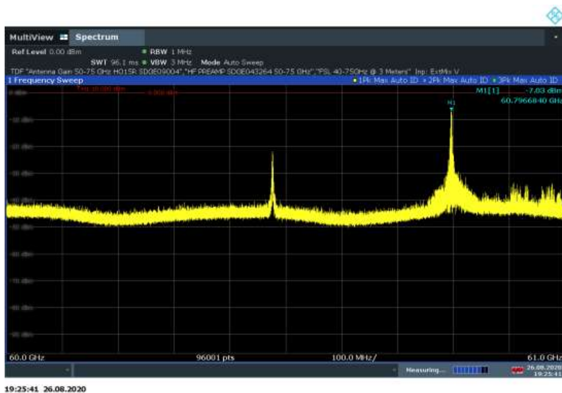
60GHz to 61GHz Plot (24 Transmitters)
