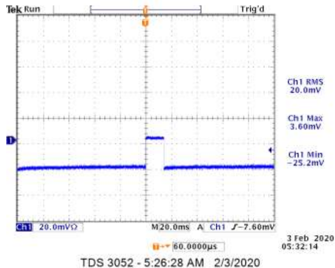
EUT (12 Transmitter) profile using a RF detector
