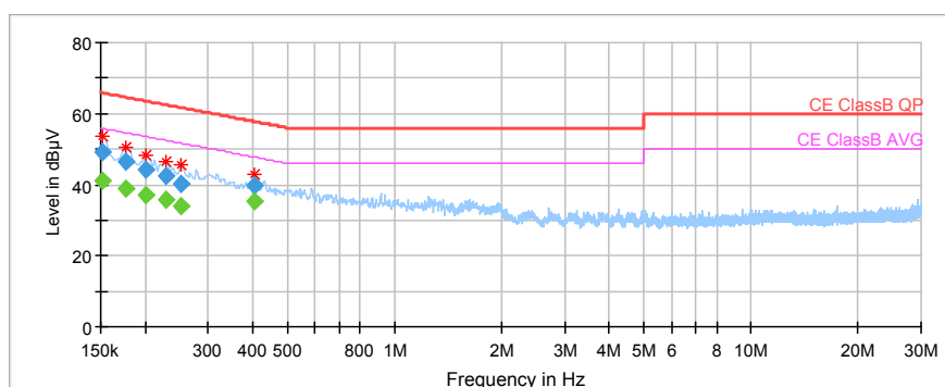
Plot 7.6.4 Conducted emission measurements
