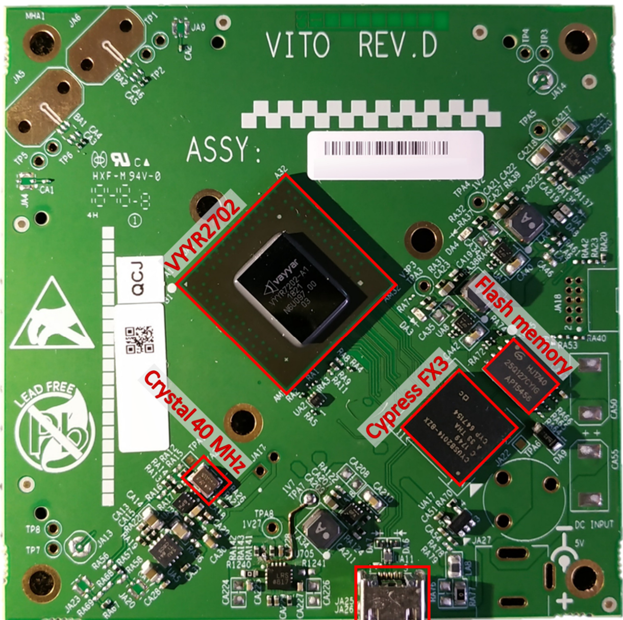
Micro USB 2.0 connector
