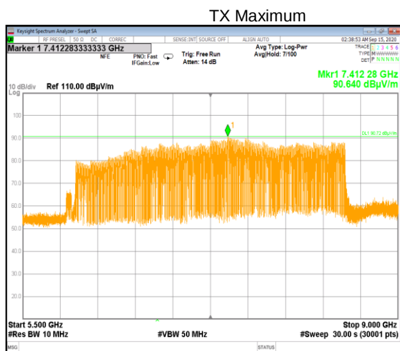
Plot 7.2.1 Peak power level contained within 50 MHz
