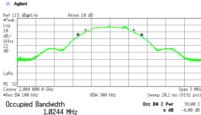
Plot 7.1.1 6 dB bandwidth test result at low frequency
