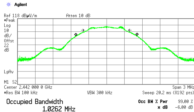
Plot 7.1.2 6 dB bandwidth test result at mid frequency
