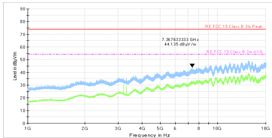
Plot 7.2.11 Radiated emission measurements from 1000 to 18000 MHz at the mid carrier frequency
