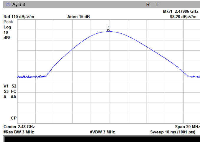
Plot 7.3.6 Field strength of carrier at high frequency
