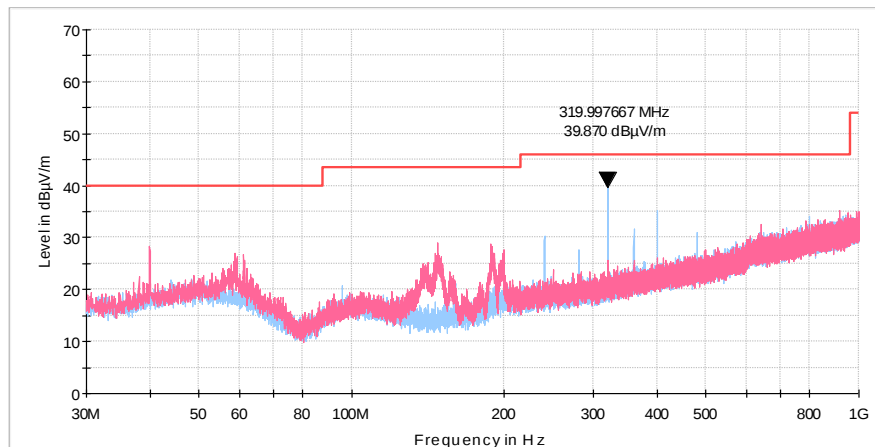
Plot 7.2.8 Radiated emission measurements from 30 to 1000 MHz at the mid carrier frequency
