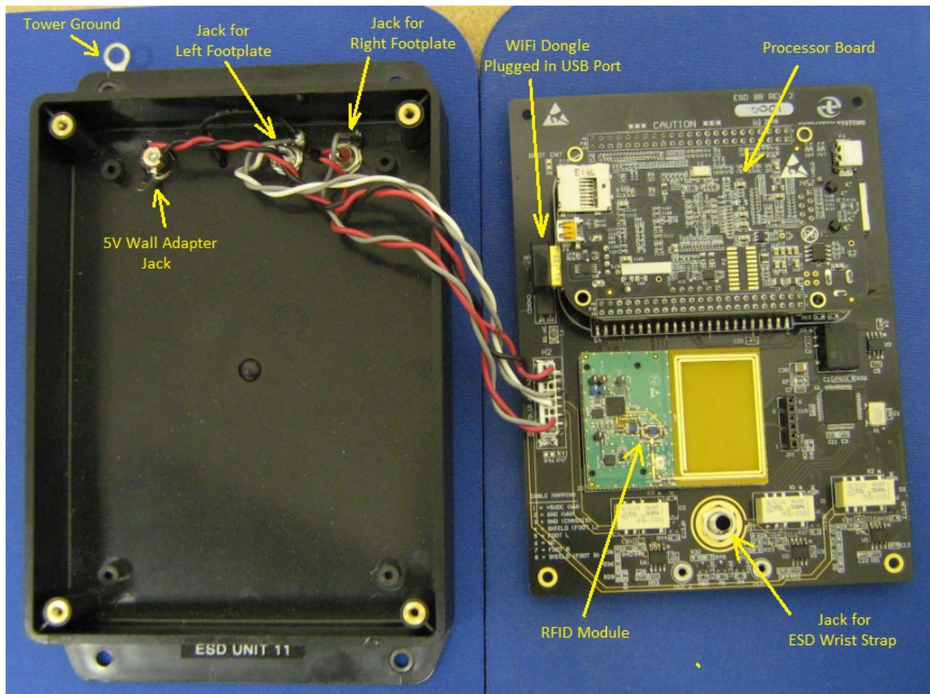
ESD Check Point Inside the ESD Tester box
