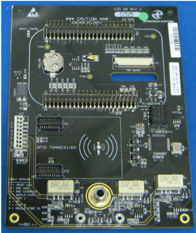
ESD BB (060-1600-50) Primary Circuit Board Bottom View
