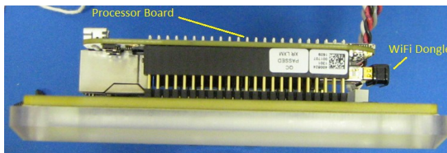
Assembled Electronics View from Top Side
