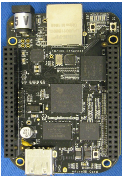
Processor Board Top View
