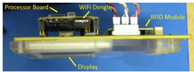
Assembled Electronics Side View
