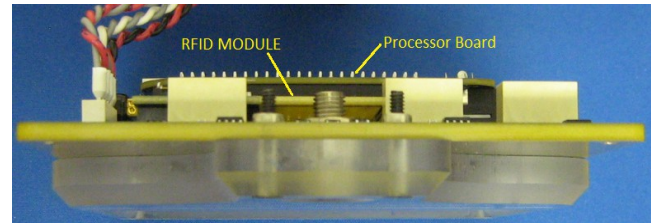
Assembled Electronics View from Bottom Side
