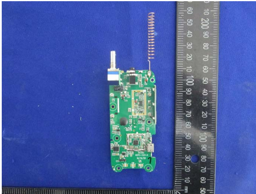
EUT – PCB Bottom Without Cover View
