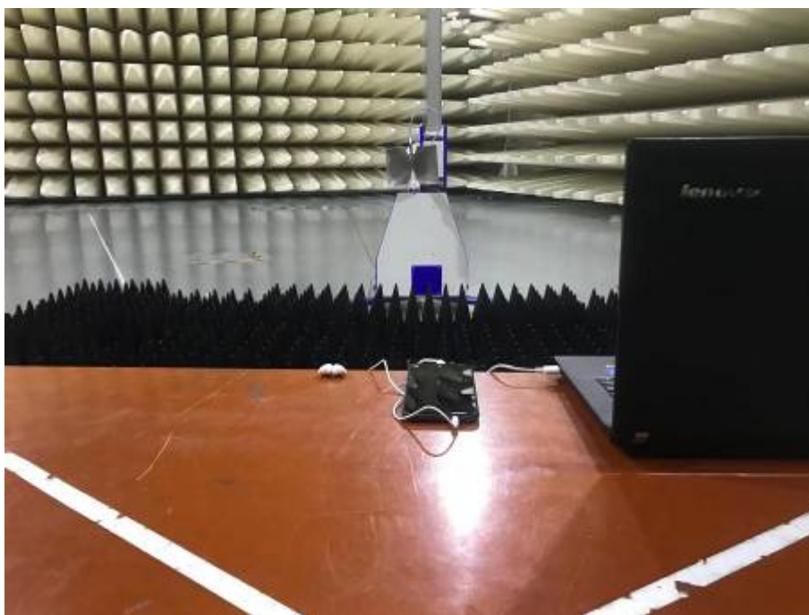
Radiated Emissions Test Setup (with laptop) (above1GHz)
