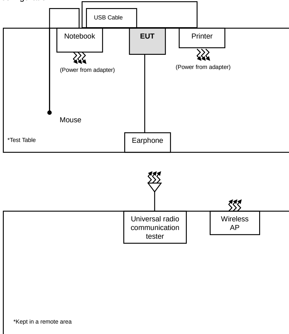
Test configuration 1
