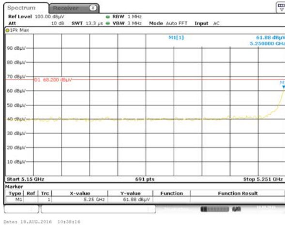
Band II 11n(HT40) CH54, PEAK
