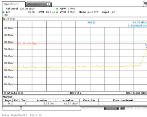
Band II 11a(HT20) CH52, PEAK
