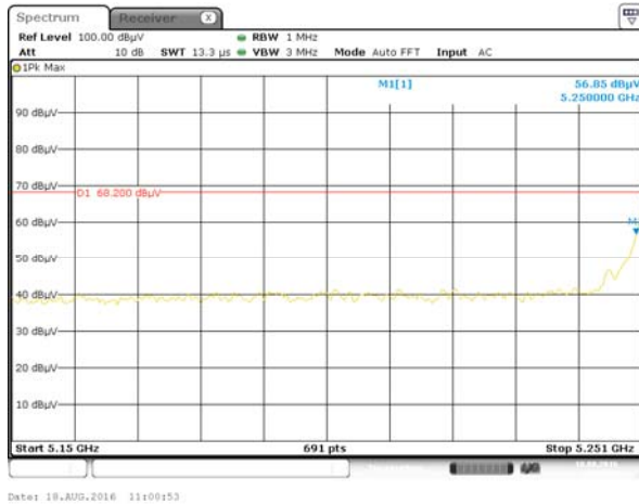
Band II 11ac(HT80) CH58, PEAK
