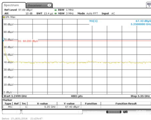
Band I 11n(HT20) CH48, PEAK
