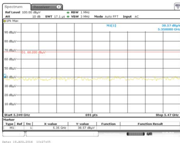
Band II 11a(HT20) CH64, PEAK
