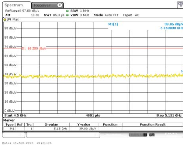
Band I 11ac(HT80) CH42, PEAK
