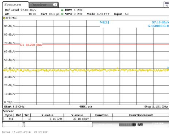
Band I 11n(HT20) CH36, PEAK
