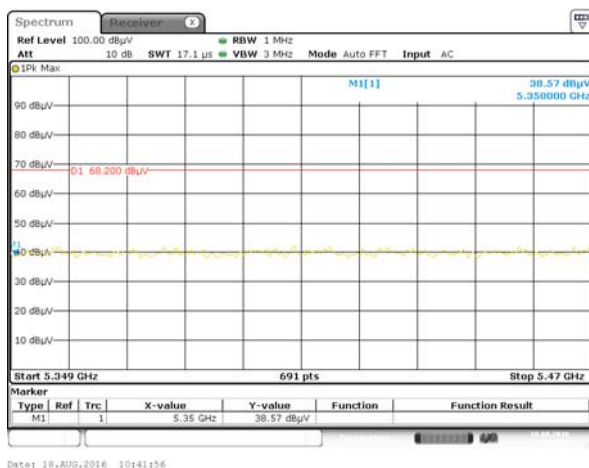
Band II 11n(HT40) CH62, PEAK
