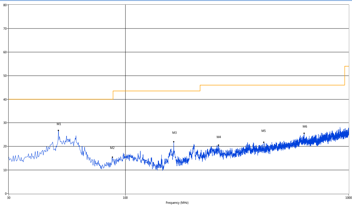
30 MHz to 1 GHz, ANT H
